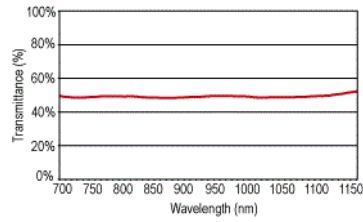
NIR 50R/50T Transmitted
