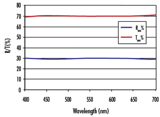
VIS 30R/70T Beamsplitter
