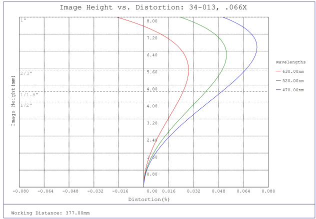
#34-013, 0.066X, 1" C-Mount TitanTL® Telecentric Lens, Distortion Plot
