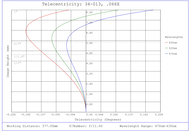
#34-013, 0.066X, 1" C-Mount TitanTL® Telecentric Lens, Telecentricity Plot
