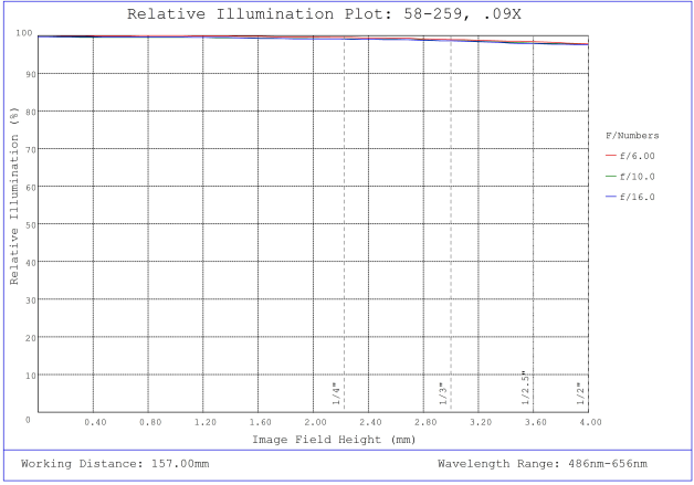
#58-259, 0.09X 1/2" GoldTL™ Telecentric Lens, Relative Illumination Plot
