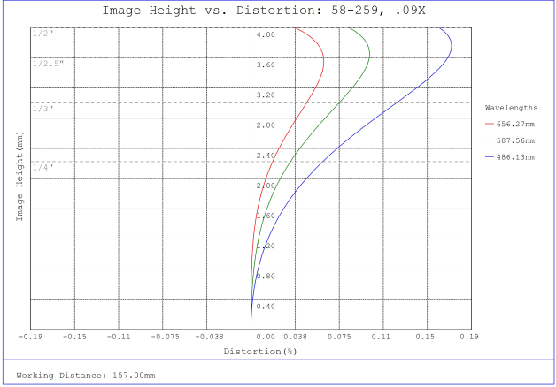
#58-259, 0.09X 1/2" GoldTL™ Telecentric Lens, Distortion Plot
