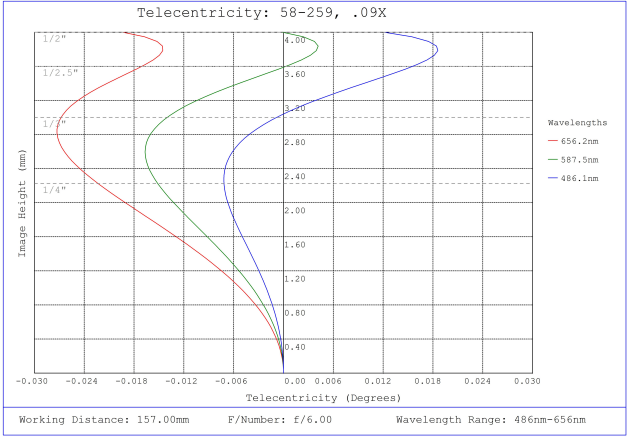
#58-259, 0.09X 1/2" GoldTL™ Telecentric Lens, Telecentricity Plot
