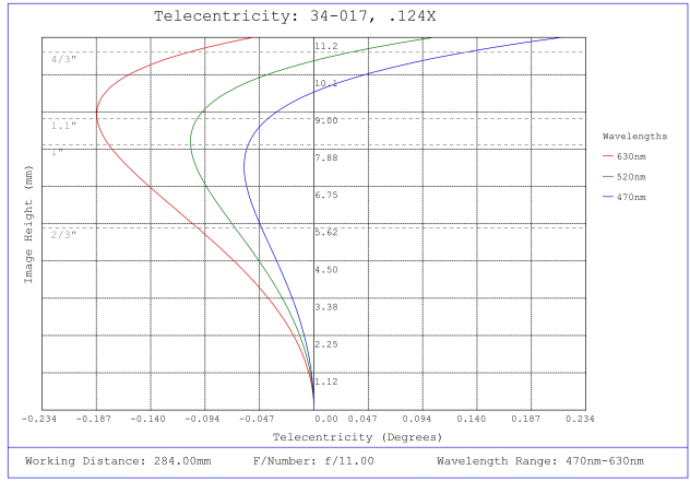
#34-017, 0.124X, 4/3" C-Mount TitanTL® Telecentric Lens, Telecentricity Plot
