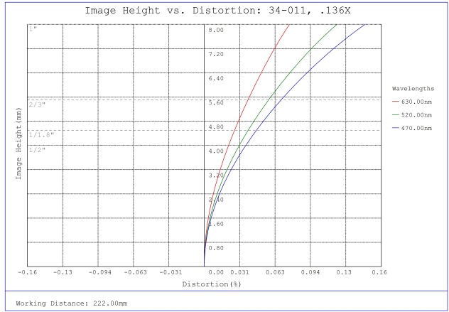
#34-011, 0.136X, 1" C-Mount TitanTL® Telecentric Lens, Distortion Plot
