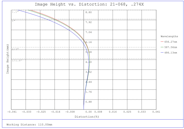
#21-068, 0.274X CobaltTL Telecentric Lens, Distortion Plot
