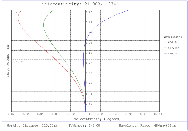
#21-068, 0.274X CobaltTL Telecentric Lens, Telecentricity Plot
