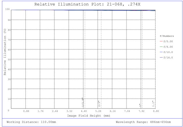
#21-068, 0.274X CobaltTL Telecentric Lens, Relative Illumination Plot
