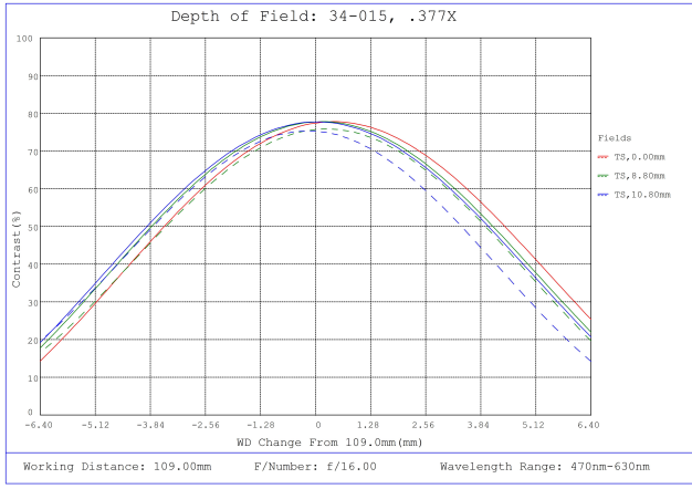
#34-015, 0.377X, 4/3" C-Mount TitanTL® Telecentric Lens, Depth of Field Plot, 109mm Working Distance, f16
