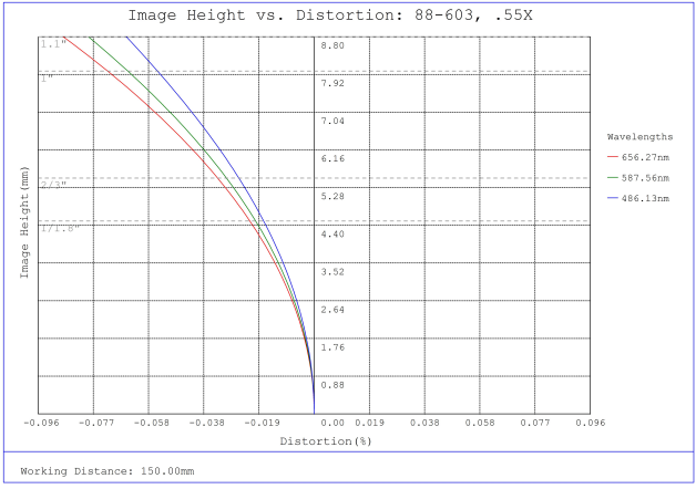
#88-603, 0.55X CobaltTL Telecentric Lens, Distortion Plot
