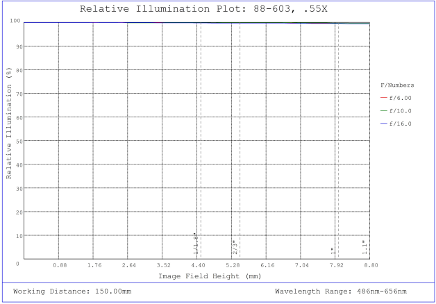
#88-603, 0.55X CobaltTL Telecentric Lens, Relative Illumination Plot
