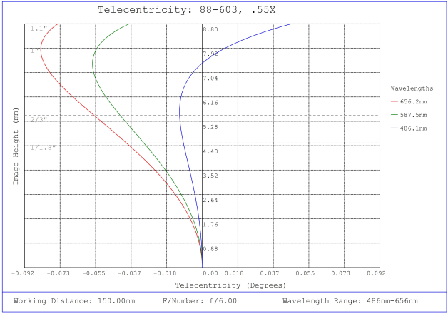
#88-603, 0.55X CobaltTL Telecentric Lens, Telecentricity Plot
