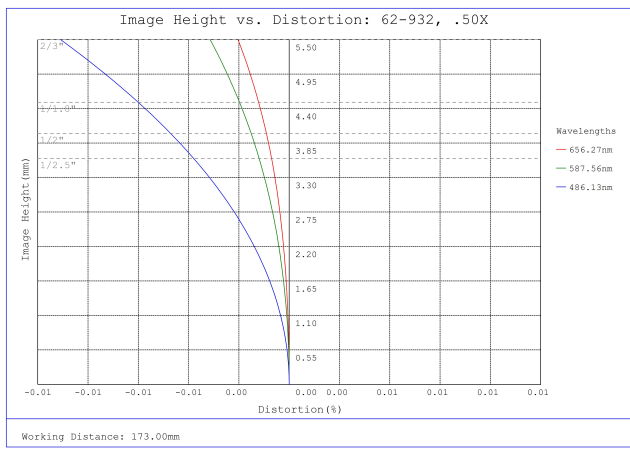
#62-932, 0.5X, 2/3" C-Mount PlatinumTL™ Telecentric Lens, Distortion Plot
