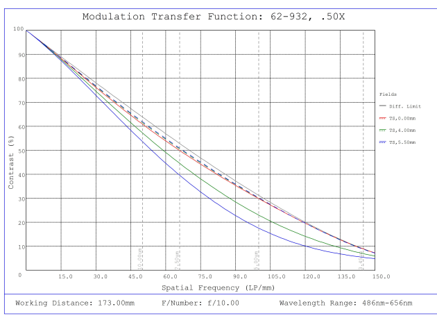
#62-932, 0.5X, 2/3" C-Mount PlatinumTL™ Telecentric Lens, Modulated Transfer Function (MTF) Plot, 173mm Working Distance, f10
