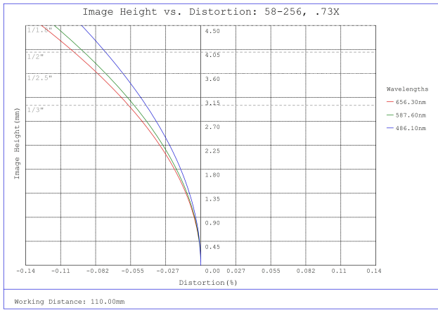
#58-256, 0.73X 1/2" GoldTL™ Telecentric Lens, Distortion Plot
