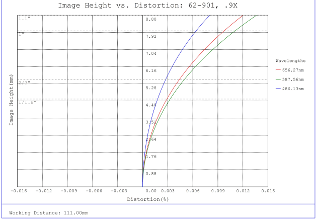
#62-901, 0.9X CobaltTL Telecentric Lens, Distortion Plot
