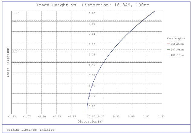
#16-849, 100mm, f/4 Athermal Lens, Distortion Plot
