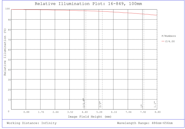
#16-849, 100mm, f/4 Athermal Lens, Relative Illumination Plot
