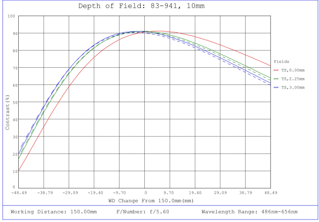
#83-941, 10mm FL f/5.6, Blue Series M12 Lens, Depth of Field Plot, 150mm Working Distance, f5.6
