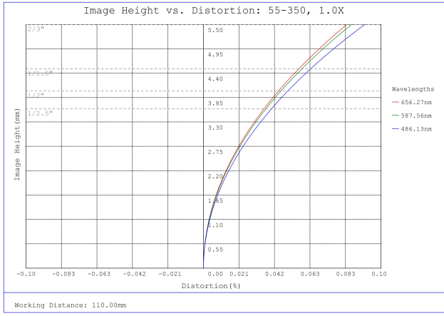
#55-350, 1.0X 2/3" GoldTL™ Telecentric Lens, Distortion Plot
