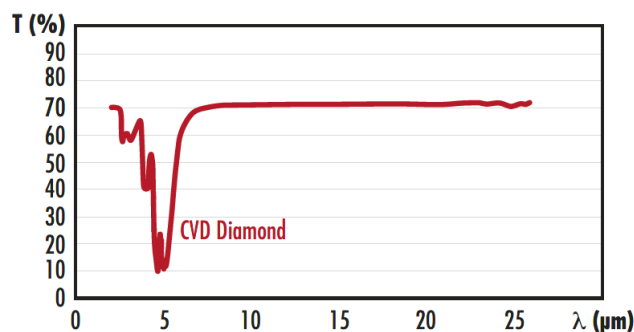
Infrared Windows Transmission
