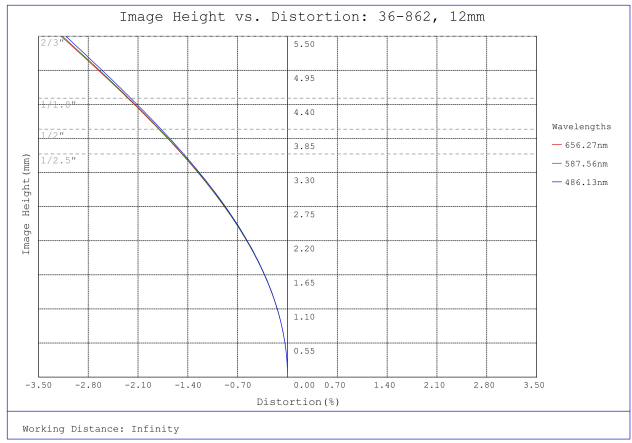
#36-862, 12mm f/11, 150-500mm Primary WD, HRr Series Fixed Focal Length Lens, Distortion Plot
