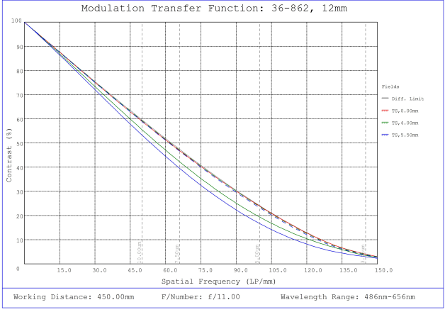
#36-862, 12mm f/11, 150-500mm Primary WD, HRr Series Fixed Focal Length Lens, Modulated Transfer Function (MTF) Plot, 450mm Working Distance, f11
