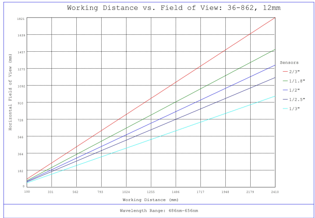
#36-862, 12mm f/11, 150-500mm Primary WD, HRr Series Fixed Focal Length Lens, Working Distance versus Field of View Plot
