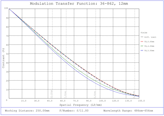
#36-862, 12mm f/11, 150-500mm Primary WD, HRr Series Fixed Focal Length Lens, Modulated Transfer Function (MTF) Plot, 250mm Working Distance, f11
