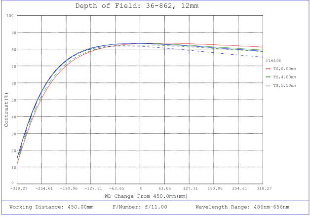
#36-862, 12mm f/11, 150-500mm Primary WD, HRr Series Fixed Focal Length Lens, Depth of Field Plot, 450mm Working Distance, f11
