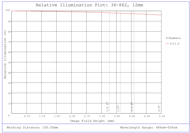
#36-862, 12mm f/11, 150-500mm Primary WD, HRr Series Fixed Focal Length Lens, Relative Illumination Plot
