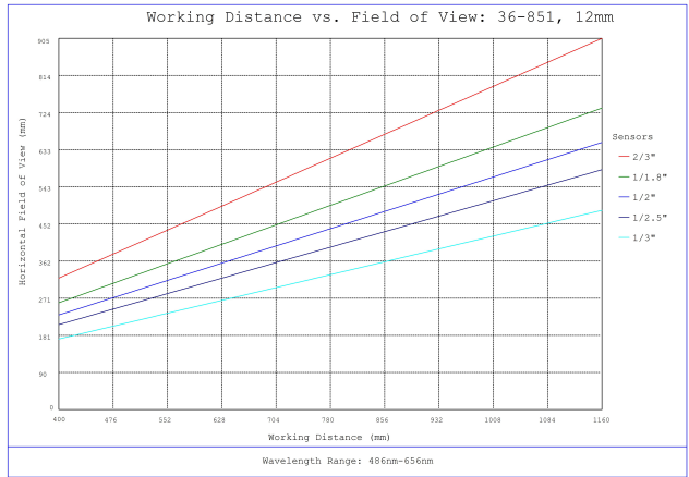
#36-851, 12mm f/2.8, 1000mm-∞ Primary WD, HRr Series Fixed Focal Length Lens, Working Distance versus Field of View Plot
