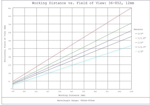
#36-852, 12mm f/4, 150-500mm Primary WD, HRr Series Fixed Focal Length Lens, Working Distance versus Field of View Plot
