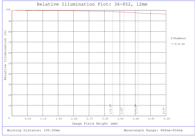
#36-852, 12mm f/4, 150-500mm Primary WD, HRr Series Fixed Focal Length Lens, Relative Illumination Plot
