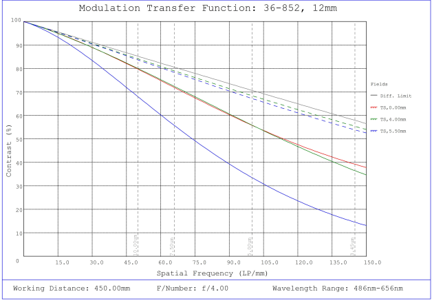
#36-852, 12mm f/4, 150-500mm Primary WD, HRr Series Fixed Focal Length Lens, Modulated Transfer Function (MTF) Plot, 450mm Working Distance, f4
