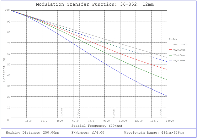
#36-852, 12mm f/4, 150-500mm Primary WD, HRr Series Fixed Focal Length Lens, Modulated Transfer Function (MTF) Plot, 250mm Working Distance, f4
