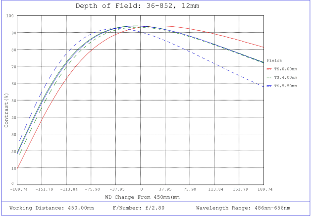
#36-852, 12mm f/4, 150-500mm Primary WD, HRr Series Fixed Focal Length Lens, Depth of Field Plot, 450mm Working Distance, f2.8
