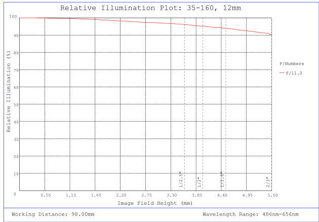
#35-160, 12mm, f/11 Cr Series Fixed Focal Length Lens, Relative Illumination Plot
