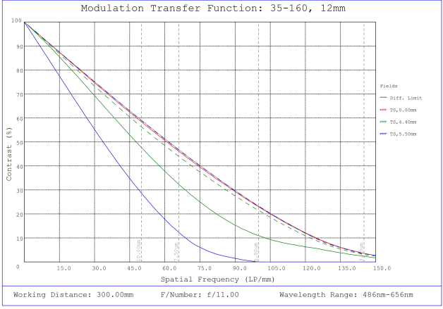
#35-160, 12mm, f/11 Cr Series Fixed Focal Length Lens, Modulated Transfer Function (MTF) Plot, 300mm Working Distance, f11
