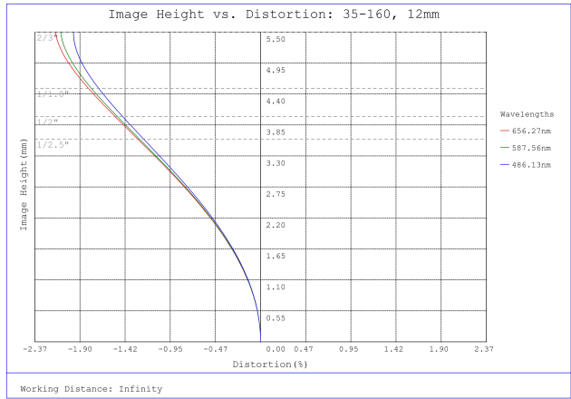
#35-160, 12mm, f/11 Cr Series Fixed Focal Length Lens, Distortion Plot
