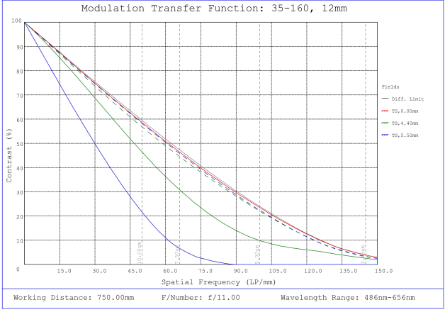
#35-160, 12mm, f/11 Cr Series Fixed Focal Length Lens, Modulated Transfer Function (MTF) Plot, 750mm Working Distance, f11
