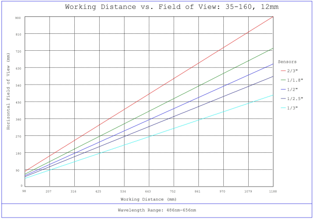
#35-160, 12mm, f/11 Cr Series Fixed Focal Length Lens, Working Distance versus Field of View Plot
