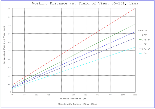
#35-161, 12mm, f/16 Cr Series Fixed Focal Length Lens, Working Distance versus Field of View Plot
