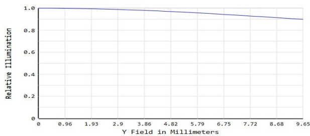
#22-835 - 12mm Focal Length, UAV Series Fixed Focal Length Lens, Relative Illumination Plot
