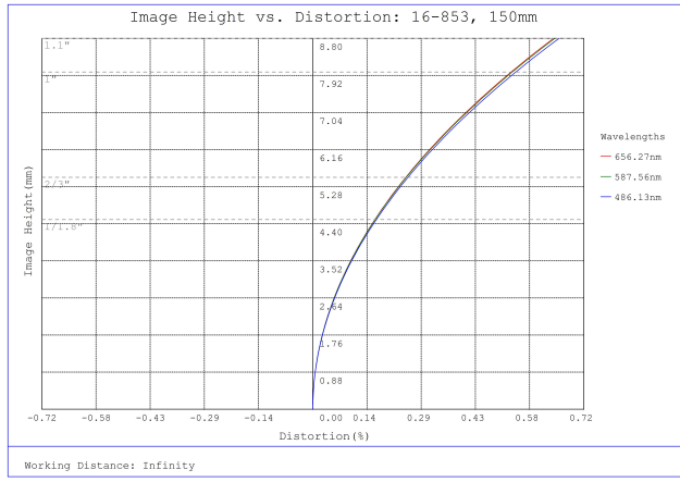
#16-853, 150mm, f/5.6 Athermal Lens, Distortion Plot
