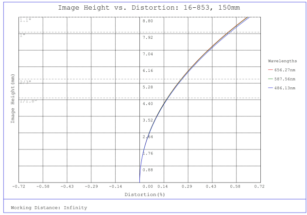
#16-853, 150mm, f/5.6 Athermal Lens, Distortion Plot
