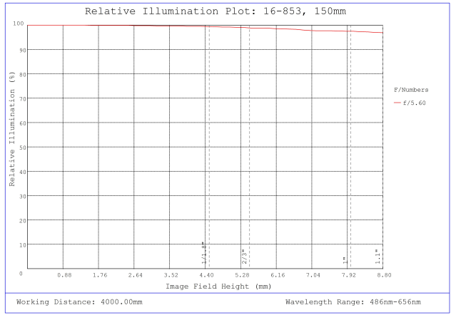
#16-853, 150mm, f/5.6 Athermal Lens, Relative Illumination Plot
