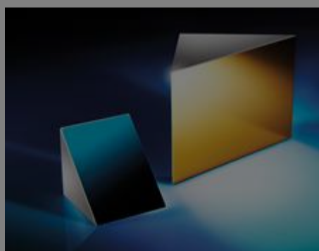
#45-592 - 10mm Enhanced Aluminum, N-BK7 Right Angle Prism Mirrors (Hypotenuse Coated) €89,00
