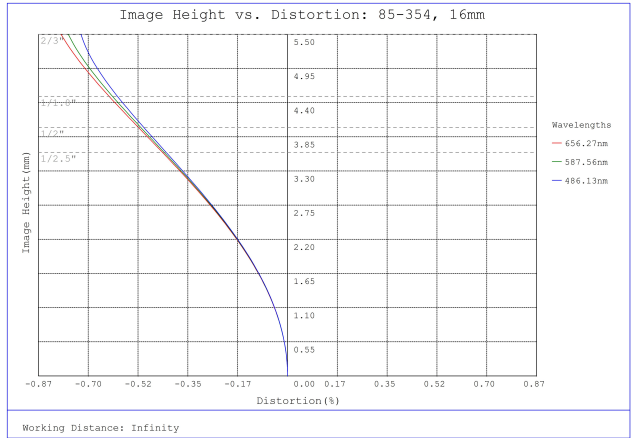
#85-354, 16mm, f/11 Ci Series Fixed Focal Length Lens, Distortion Plot
