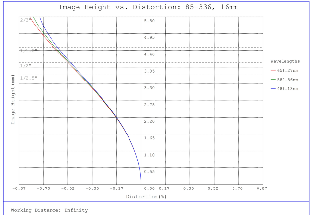
#85-336, 16mm, f/16 Ci Series Fixed Focal Length Lens, Distortion Plot
