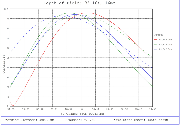
#35-164, 16mm, f/1.8 Cr Series Fixed Focal Length Lens, Depth of Field Plot, 500mm Working Distance, f1.8
