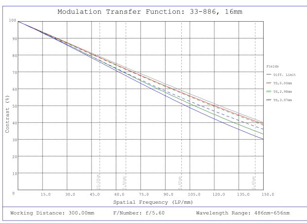
#33-886, 16mm, f/5.6 UCI Series Fixed Focal Length Lens, Modulated Transfer Function (MTF) Plot, 300mm Working Distance, f5.6
