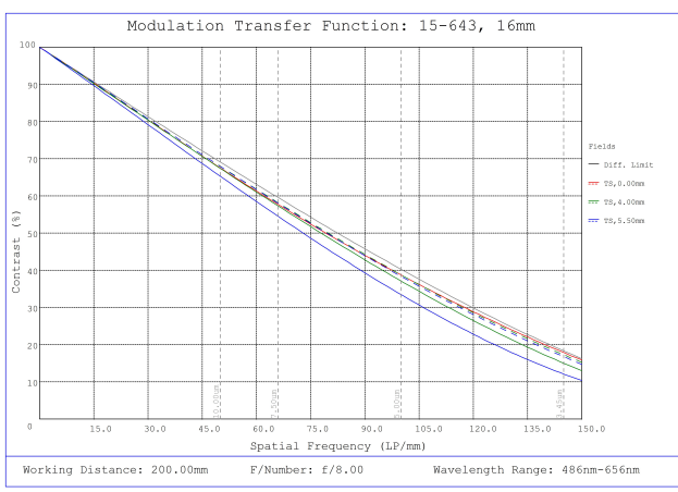
#15-643, 16mm, f/8 Cw Series Fixed Focal Length Lens, Modulated Transfer Function (MTF) Plot, 200mm Working Distance, f8
