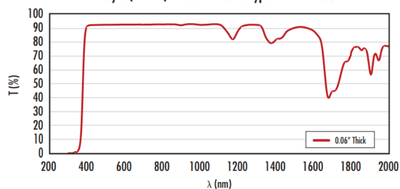
Acrylic (PMMA) Plastic Windows Typical Transmission
