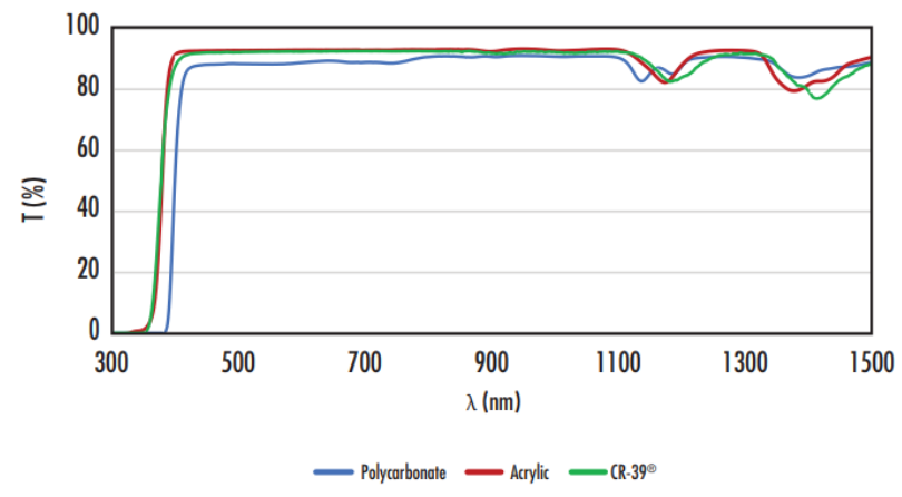
Typical Transmission of Plastic Windows
