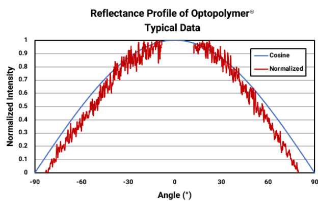
Typical, normalized reflectance profile of Optopolymer®, showing near Lambertian properties. The gap in data is due to the detector crossing the path of the incident beam.
