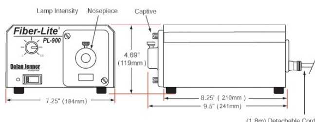
Dolan-Jenner Illuminator
