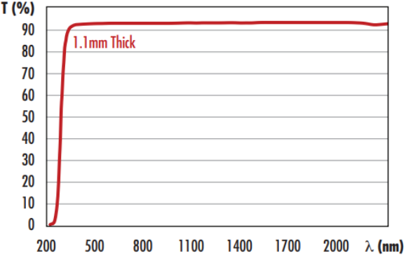
Gorilla® Glass 3 Typical Transmission
