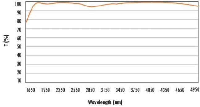
Calcium Fluoride with 2000-5000nm BBAR Coating Typical Transmission
