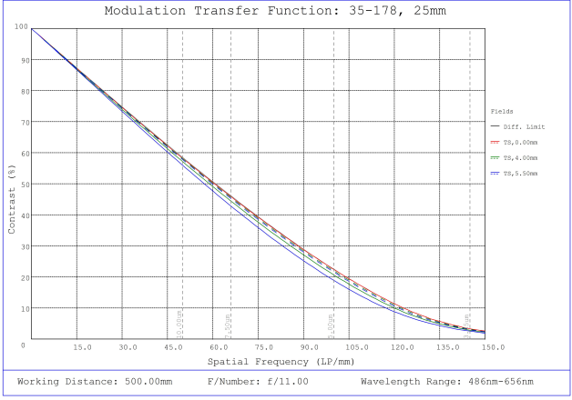
#35-178, 25mm, f/11 Cr Series Fixed Focal Length Lens, Modulated Transfer Function (MTF) Plot, 500mm Working Distance, f11
