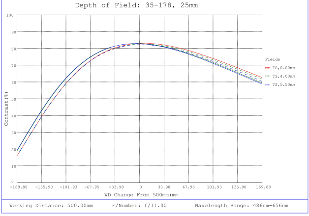
#35-178, 25mm, f/11 Cr Series Fixed Focal Length Lens, Depth of Field Plot, 500mm Working Distance, f11
