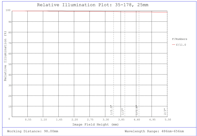
#35-178, 25mm, f/11 Cr Series Fixed Focal Length Lens, Relative Illumination Plot
