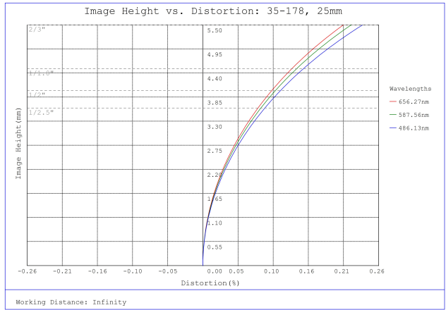
#35-178, 25mm, f/11 Cr Series Fixed Focal Length Lens, Distortion Plot
