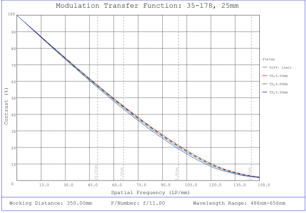
#35-178, 25mm, f/11 Cr Series Fixed Focal Length Lens, Modulated Transfer Function (MTF) Plot, 350mm Working Distance, f11
