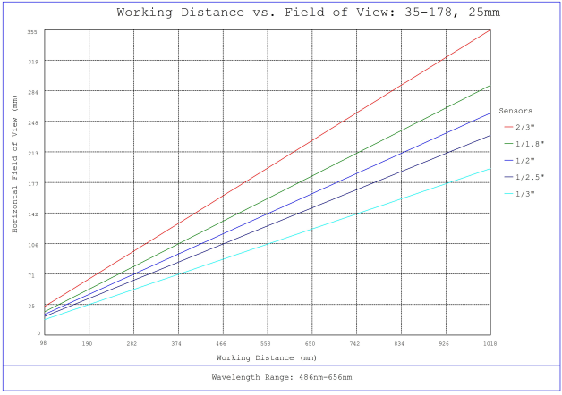
#35-178, 25mm, f/11 Cr Series Fixed Focal Length Lens, Working Distance versus Field of View Plot
