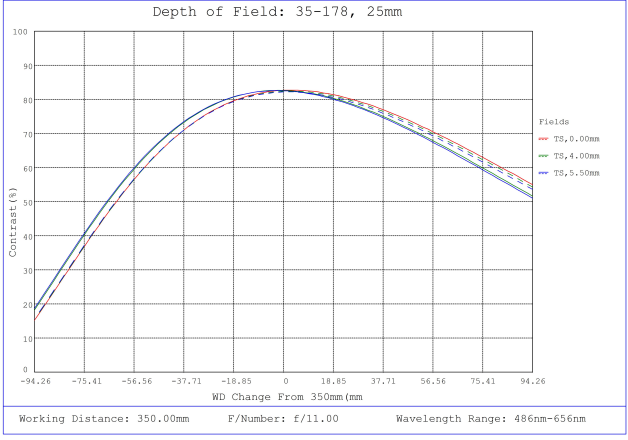
#35-178, 25mm, f/11 Cr Series Fixed Focal Length Lens, Depth of Field Plot, 350mm Working Distance, f11
