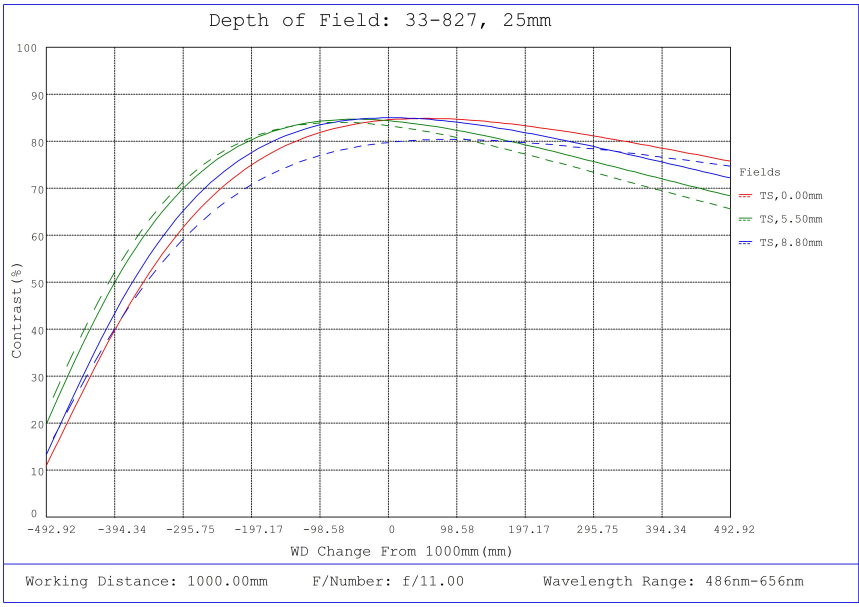
#33-827, 25mm f/11.0, HPI Series Fixed Focal Length Lens, Depth of Field Plot, 1000mm Working Distance, f11
