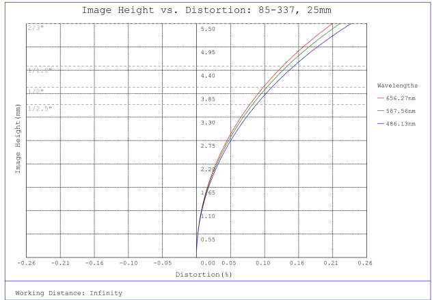
#85-337, 25mm, f/16 Ci Series Fixed Focal Length Lens, Distortion Plot
