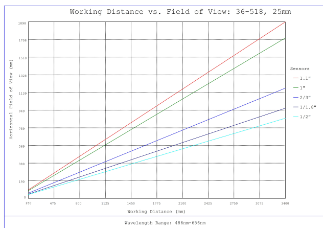
#36-518, 25mm f/1.8, HPr Series Fixed Focal Length Lens, Working Distance versus Field of View Plot
