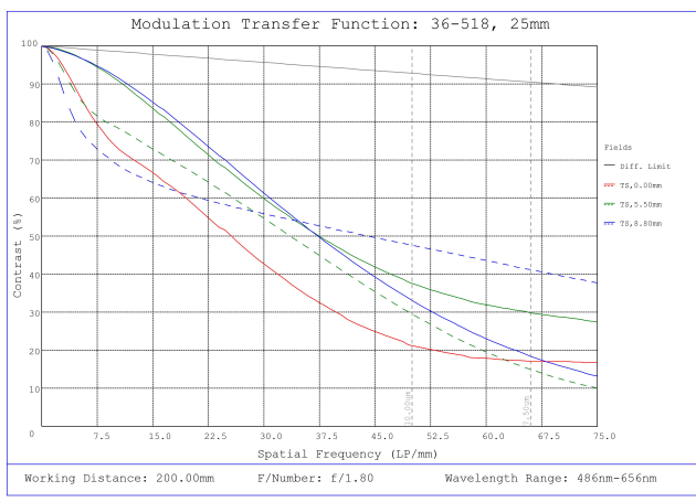
#36-518, 25mm f/1.8, HPr Series Fixed Focal Length Lens, Modulated Transfer Function (MTF) Plot, 200mm Working Distance, f1.8
