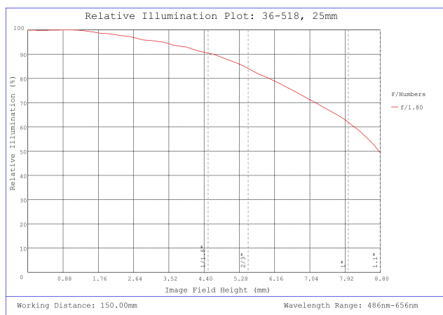
#36-518, 25mm f/1.8, HPr Series Fixed Focal Length Lens, Relative Illumination Plot
