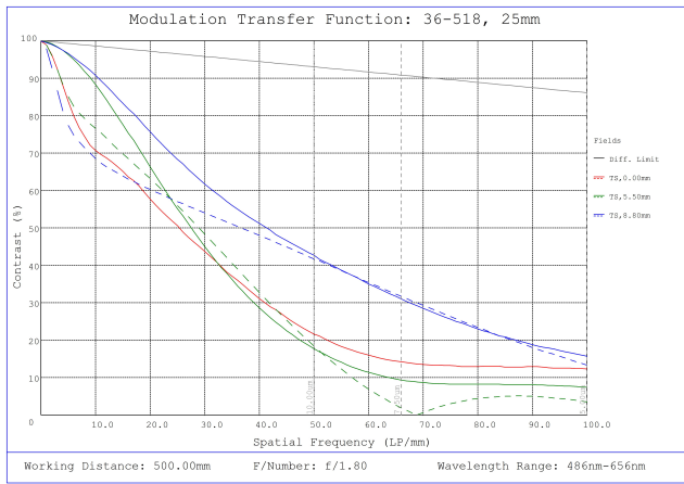
#36-518, 25mm f/1.8, HPr Series Fixed Focal Length Lens, Modulated Transfer Function (MTF) Plot, 500mm Working Distance, f1.8
