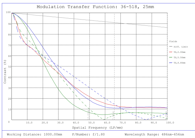
#36-518, 25mm f/1.8, HPr Series Fixed Focal Length Lens, Modulated Transfer Function (MTF) Plot, 1000mm Working Distance, f1.8
