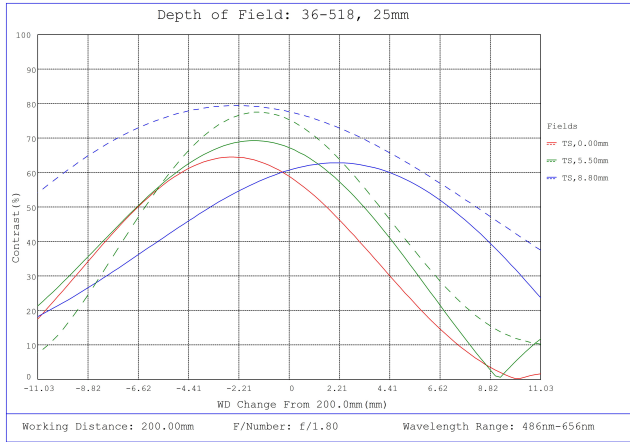
#36-518, 25mm f/1.8, HPr Series Fixed Focal Length Lens, Depth of Field Plot, 200mm Working Distance, f1.8
