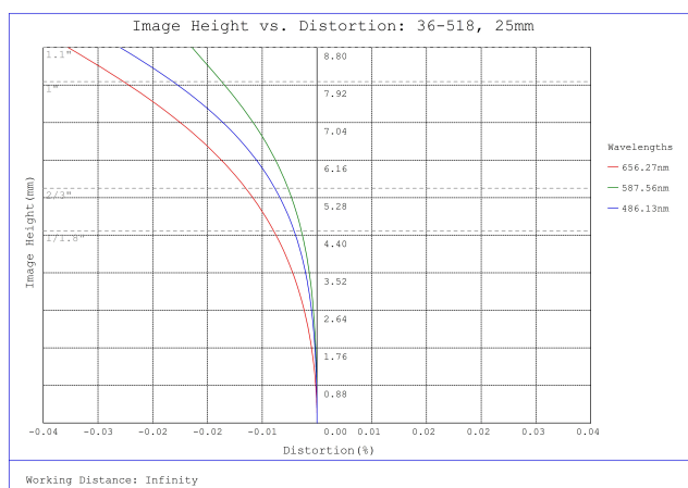
#36-518, 25mm f/1.8, HPr Series Fixed Focal Length Lens, Distortion Plot
