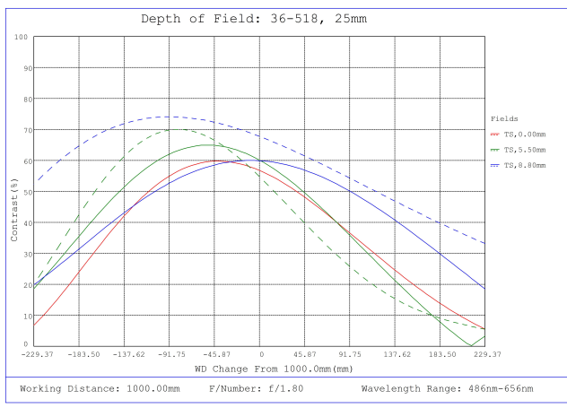
#36-518, 25mm f/1.8, HPr Series Fixed Focal Length Lens, Depth of Field Plot, 1000mm Working Distance, f1.8
