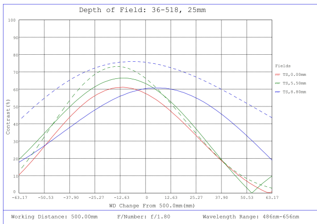
#36-518, 25mm f/1.8, HPr Series Fixed Focal Length Lens, Depth of Field Plot, 500mm Working Distance, f1.8
