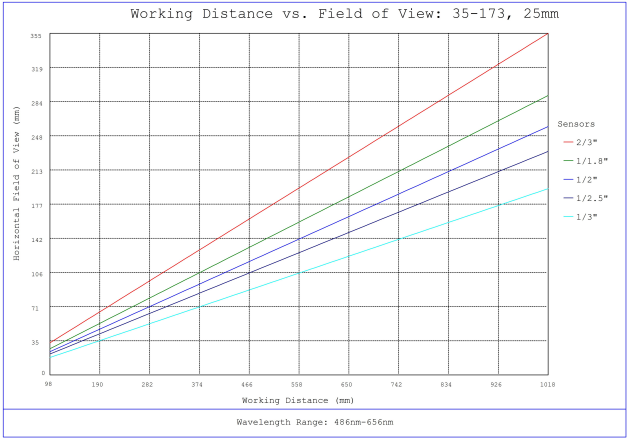
#35-173, 25mm, f/1.8 Cr Series Fixed Focal Length Lens, Working Distance versus Field of View Plot
