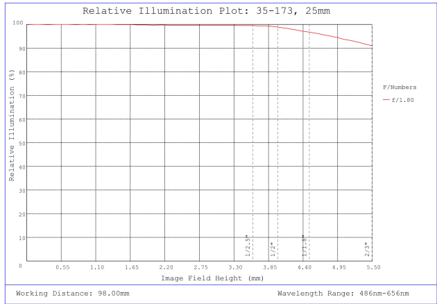
#35-173, 25mm, f/1.8 Cr Series Fixed Focal Length Lens, Relative Illumination Plot
