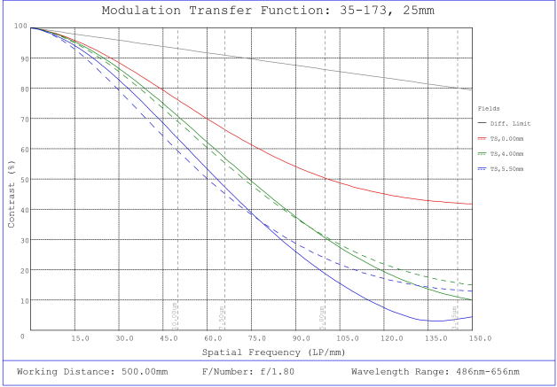
#35-173, 25mm, f/1.8 Cr Series Fixed Focal Length Lens, Modulated Transfer Function (MTF) Plot, 500mm Working Distance, f1.8
