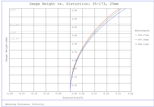
#35-173, 25mm, f/1.8 Cr Series Fixed Focal Length Lens, Distortion Plot
