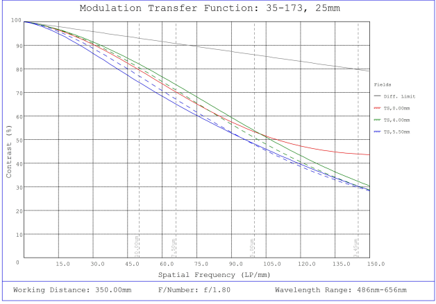
#35-173, 25mm, f/1.8 Cr Series Fixed Focal Length Lens, Modulated Transfer Function (MTF) Plot, 350mm Working Distance, f1.8
