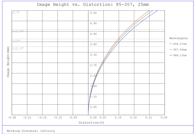
#85-357, 25mm, f/2.8 Ci Series Fixed Focal Length Lens, Distortion Plot
