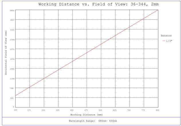
#36-344, 2mm FL f/4 Rugged Blue Series M12 Lens, Working Distance versus Field of View Plot
