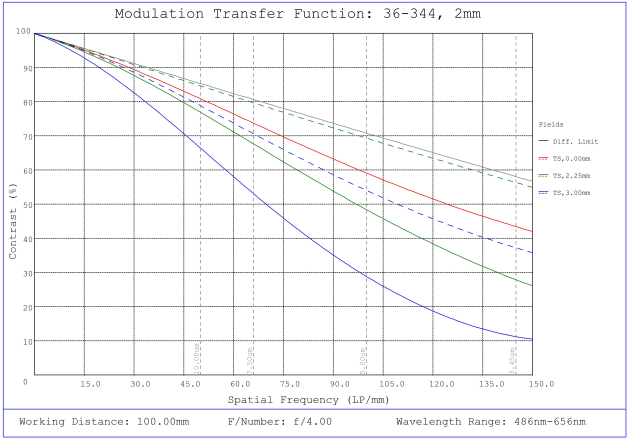
#36-344, 2mm FL f/4 Rugged Blue Series M12 Lens, Modulated Transfer Function (MTF) Plot, 100mm Working Distance, f4
