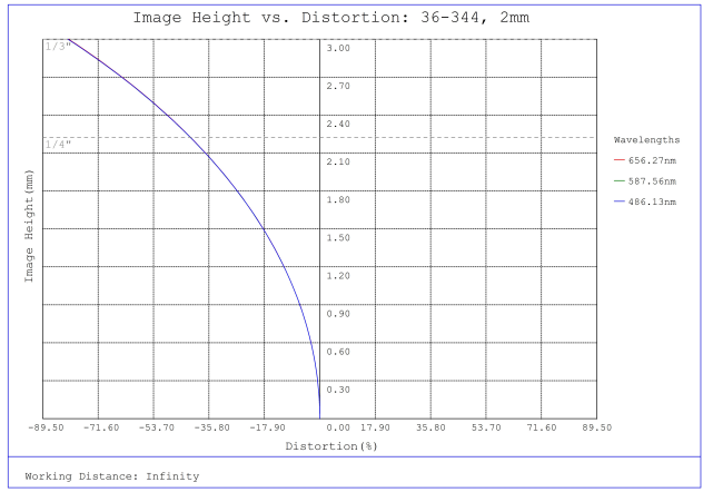
#36-344, 2mm FL f/4 Rugged Blue Series M12 Lens, Distortion Plot
