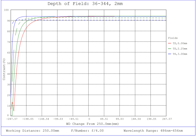
#36-344, 2mm FL f/4 Rugged Blue Series M12 Lens, Depth of Field Plot, 250mm Working Distance, f4
