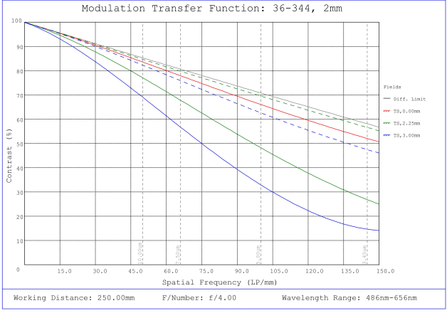
#36-344, 2mm FL f/4 Rugged Blue Series M12 Lens, Modulated Transfer Function (MTF) Plot, 250mm Working Distance, f4
