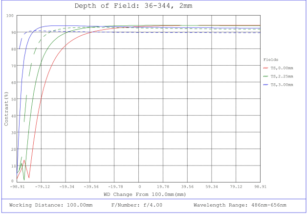
#36-344, 2mm FL f/4 Rugged Blue Series M12 Lens, Depth of Field Plot, 100mm Working Distance, f4
