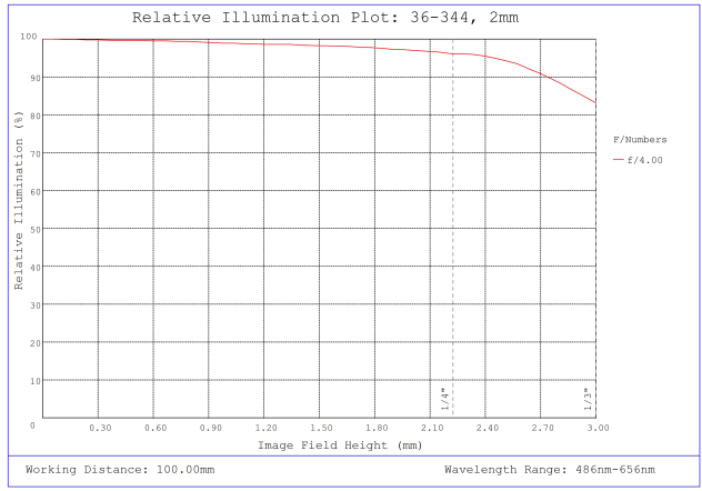
#36-344, 2mm FL f/4 Rugged Blue Series M12 Lens, Relative Illumination Plot
