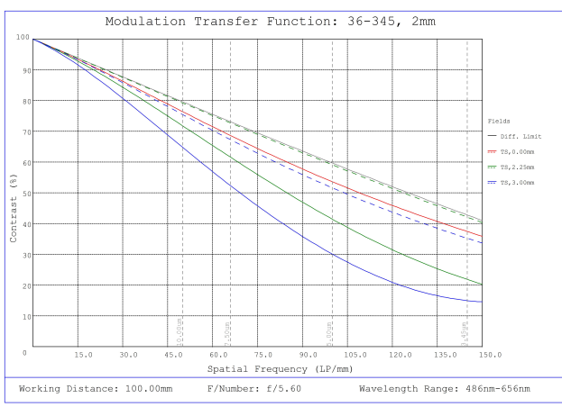
#36-345, 2mm FL f/5.6 Rugged Blue Series M12 Lens, Modulated Transfer Function (MTF) Plot, 100mm Working Distance, f5.6
