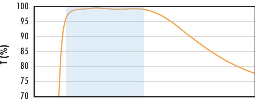
N-BK7 with VIS-EXT Coating Typical Transmission
