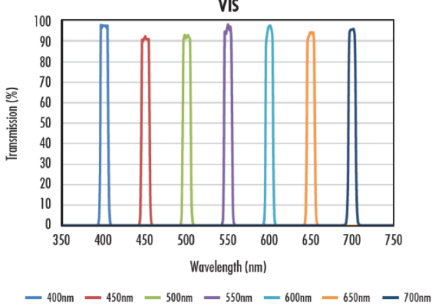
TECHSPEC® Hard Coated OD 4.0 10nm Bandpass Filters
