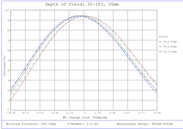
#35-183, 35mm, f/2.8 Cr Series Fixed Focal Length Lens, Depth of Field Plot, 300mm Working Distance, f2.8
