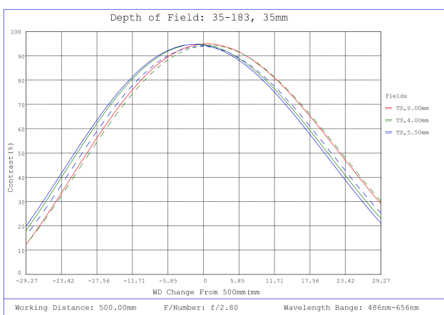
#35-183, 35mm, f/2.8 Cr Series Fixed Focal Length Lens, Depth of Field Plot, 500mm Working Distance, f2.8
