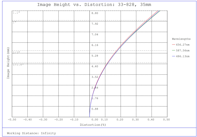
#33-828, 35mm f/1.8, HPI Series Fixed Focal Length Lens, Distortion Plot
