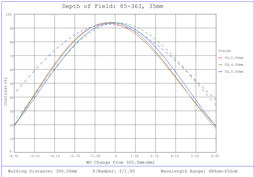
#85-363, 35mm, f/1.8 Ci Series Fixed Focal Length Lens, Depth of Field Plot, 300mm Working Distance, f1.8
