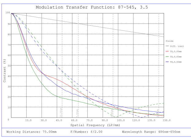
#87-545, 3.5mm, f/2 Ci Series Fixed Focal Length Lens, Modulated Transfer Function (MTF) Plot, 75mm Working Distance, f2
