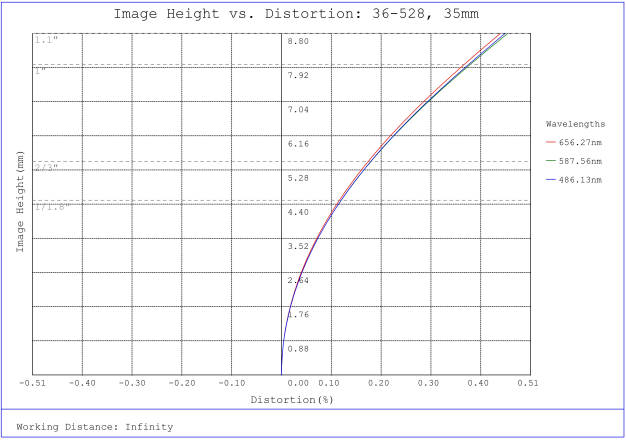
#36-528, 35mm f/4.0, HPr Series Fixed Focal Length Lens, Distortion Plot
