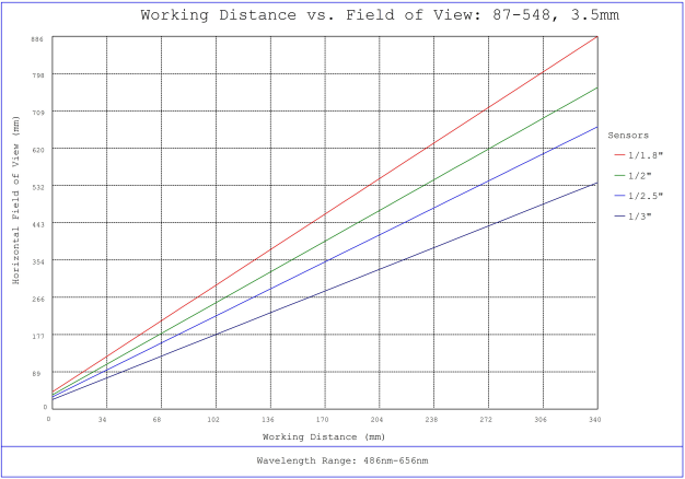
#87-548, 3.5mm, f/5.6 Ci Series Fixed Focal Length Lens, Working Distance versus Field of View Plot
