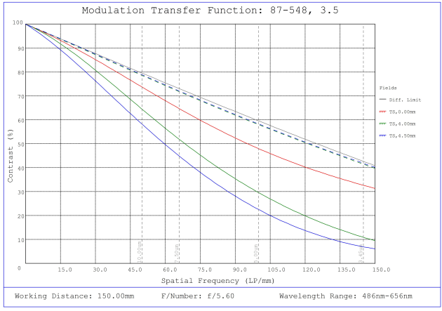
#87-548, 3.5mm, f/5.6 Ci Series Fixed Focal Length Lens, Modulated Transfer Function (MTF) Plot, 150mm Working Distance, f5.6
