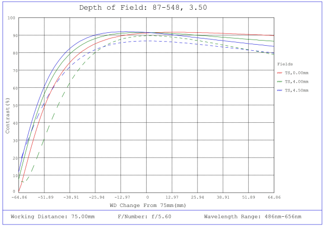
#87-548, 3.5mm, f/5.6 Ci Series Fixed Focal Length Lens, Depth of Field Plot, 75mm Working Distance, f5.6
