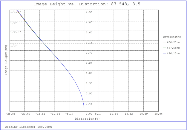
#87-548, 3.5mm, f/5.6 Ci Series Fixed Focal Length Lens, Distortion Plot
