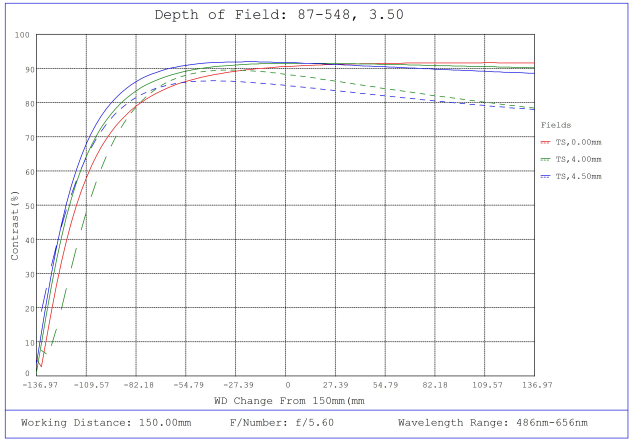
#87-548, 3.5mm, f/5.6 Ci Series Fixed Focal Length Lens, Depth of Field Plot, 150mm Working Distance, f5.6
