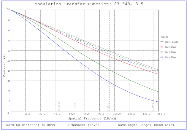
#87-548, 3.5mm, f/5.6 Ci Series Fixed Focal Length Lens, Modulated Transfer Function (MTF) Plot, 75mm Working Distance, f5.6
