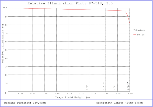
#87-548, 3.5mm, f/5.6 Ci Series Fixed Focal Length Lens, Relative Illumination Plot
